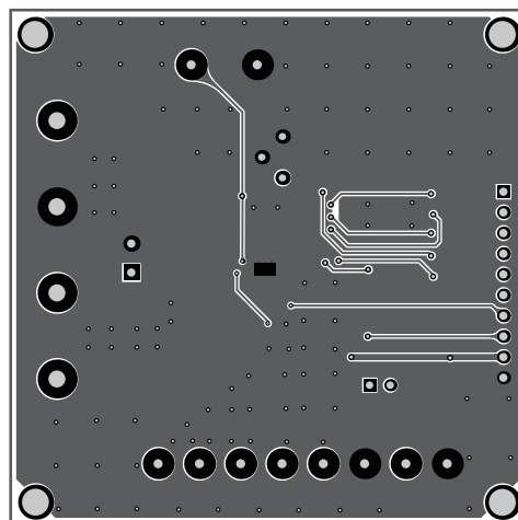
Figure 3: Bottom Layer
