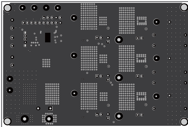
Figure 3: Inner1
