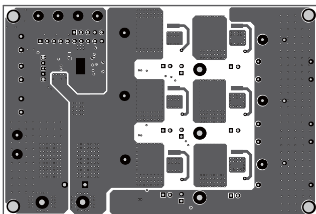
Figure 5: Bottom
