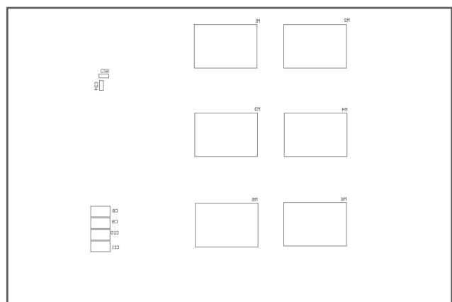
Figure 6: Bottom Silk
