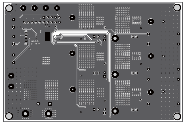
Figure 4:Inner2
