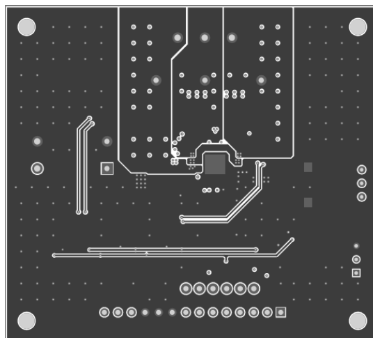
Figure 4—Inner 2 Layer
