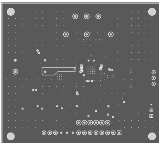
Figure 3—Inner 1 Layer
