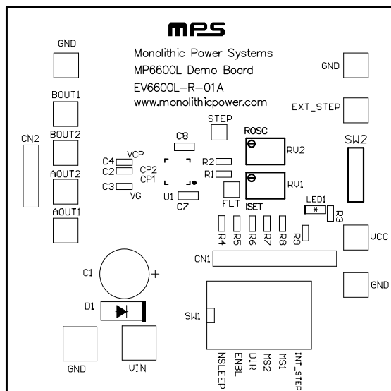
Figure 2: Top Silk
