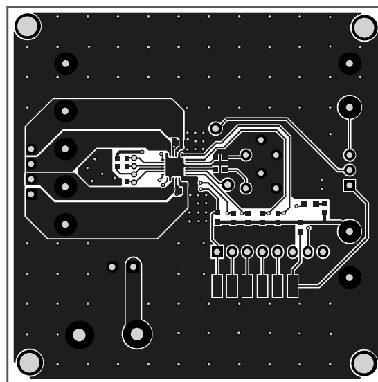
Figure 3: Top Layer
