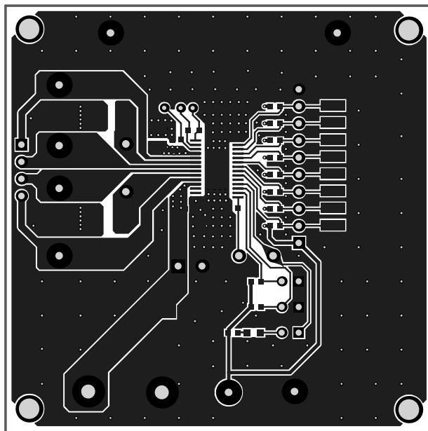
Figure 3: Top Layer
