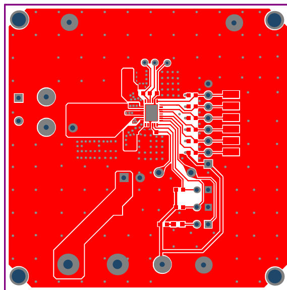
Figure 4: Top Layer
