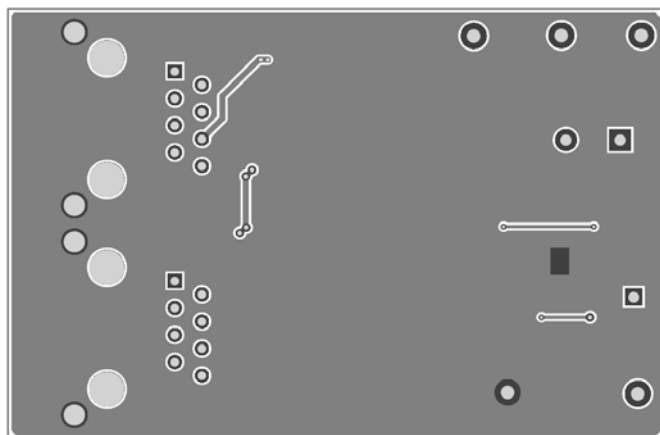
Figure 3: Bottom Layer
