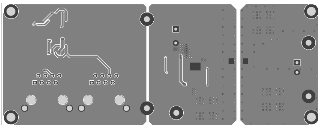
Figure 3: Bottom Layer
