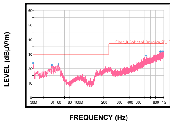
Radiated Emissions Results
