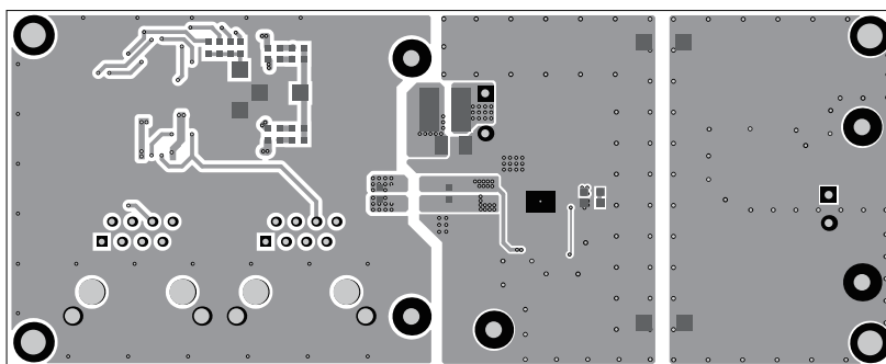
Figure 5: Bottom Layer
