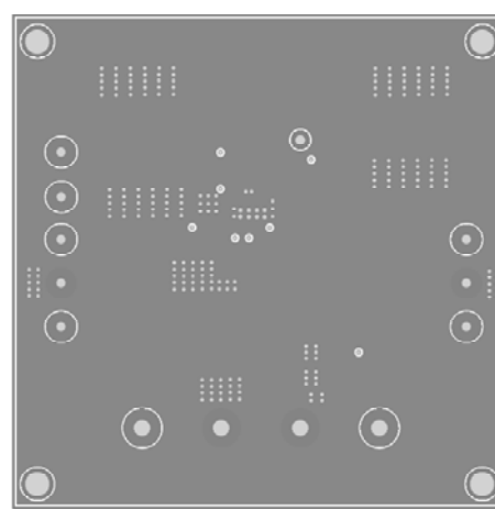
Figure 4—Inner2 Layer
