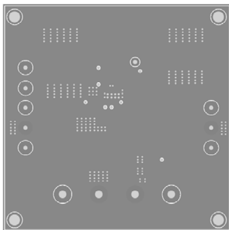
Figure 3—Inner1 Layer
