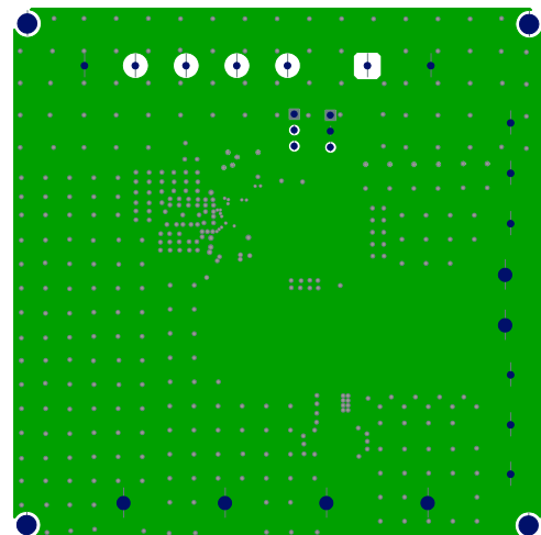
Figure 2—Inner Layer 1
