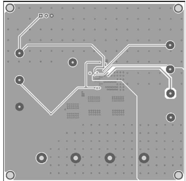
Figure 4: Inner Layer2
