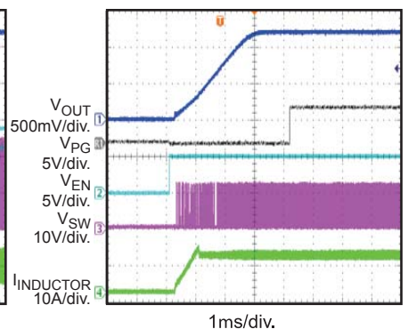
Start-Up through V_{EN}
