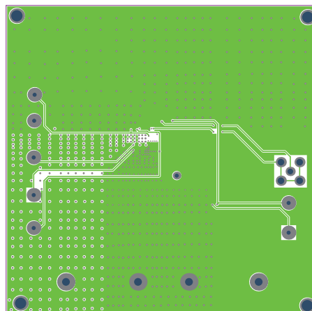
Figure 4—Inner Layer 2
