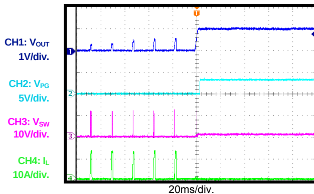
Short Circuit Protection Recovery I_{OUT}=0A
