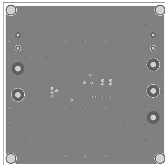
Figure 4: Inner Layer 1
