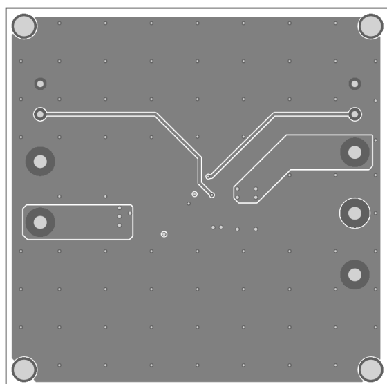
Figure 5: Inner Layer 2
