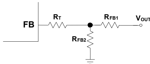
Figure 1: T-Type Network
