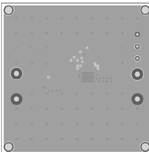
Figure 5: Bottom Layer
