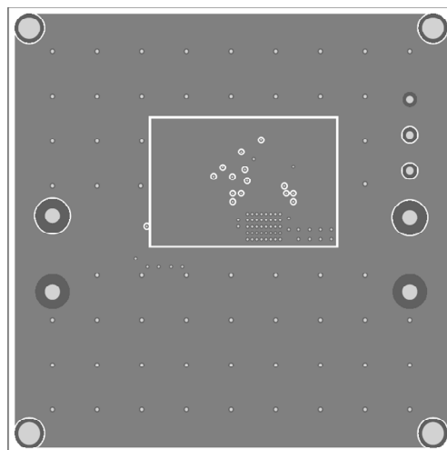
Figure 3: Mid-Layer 1
