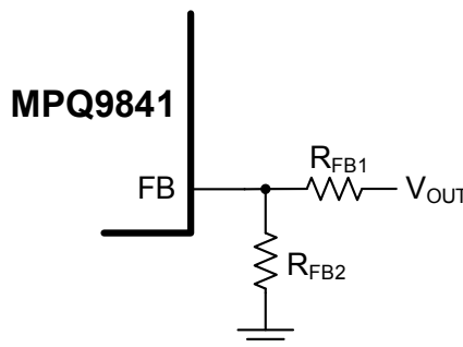
Figure 1: Feedback Circuit
