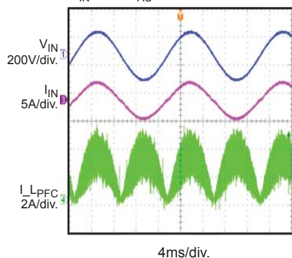
Input Voltage & Current
