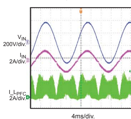
Input Voltage & Current
