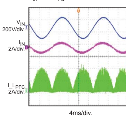
Input Voltage & Current
