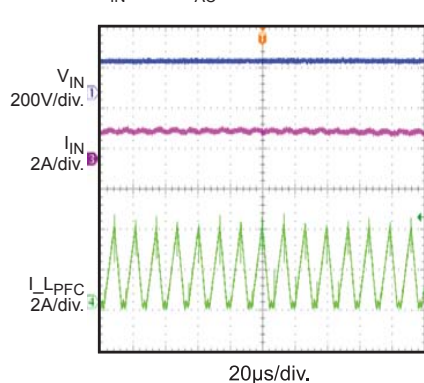
PFC Stage
