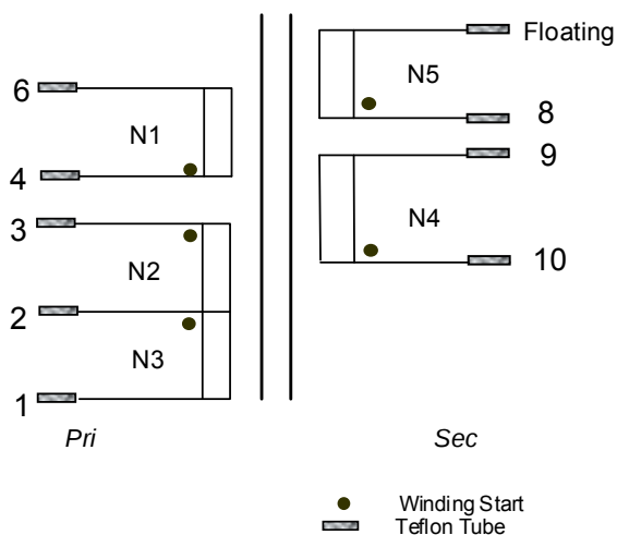
Electrical Diagram
