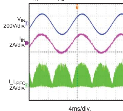
Input Voltage & Current
