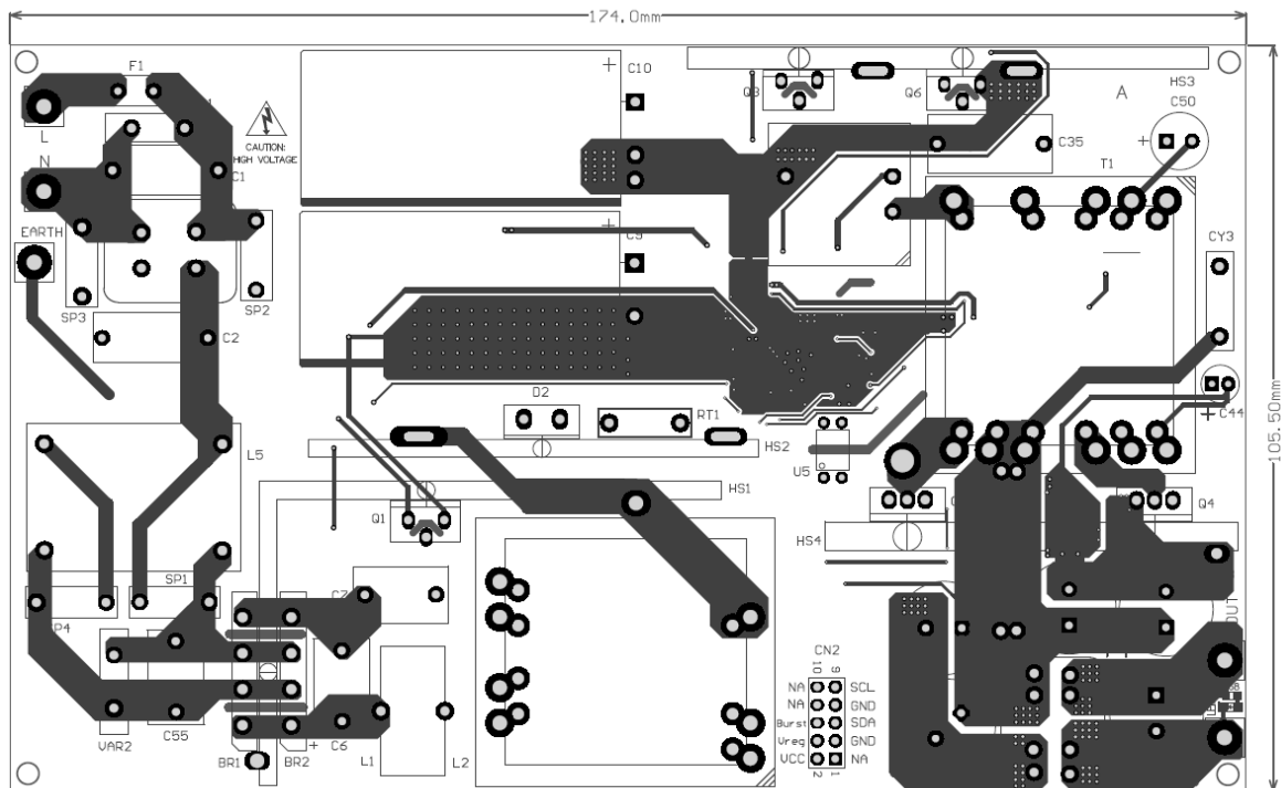
Figure 1: Top Layer
