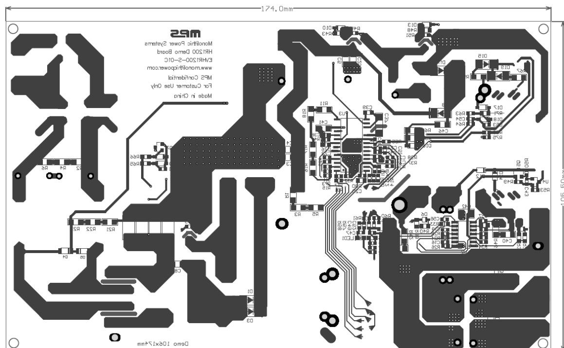
Figure 2: Bottom Layer
