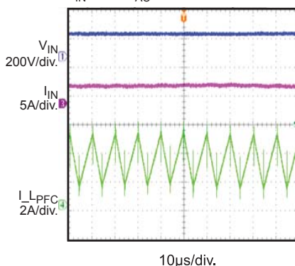
PFC Stage
