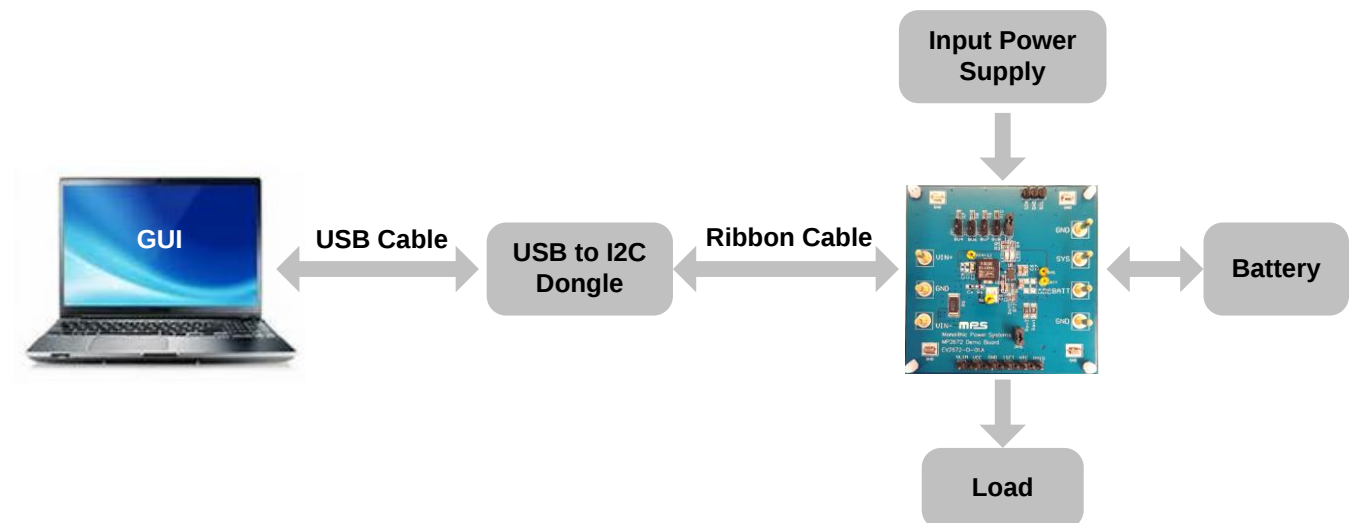
Figure 1: EVKT-MP2672 Evaluation Kit Set-Up
