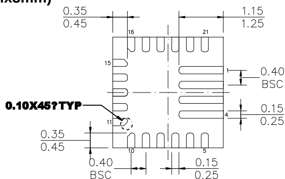
QFN-21 (3mmx3mm)
