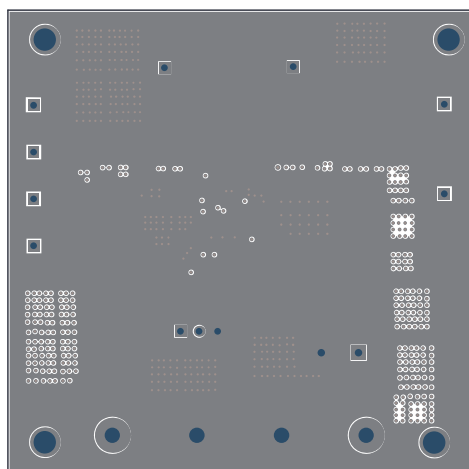
Figure 4: Mid-Layer 1
