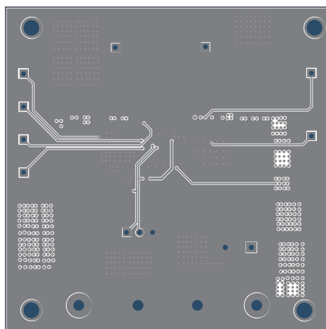
Figure 5: Mid-Layer 2
