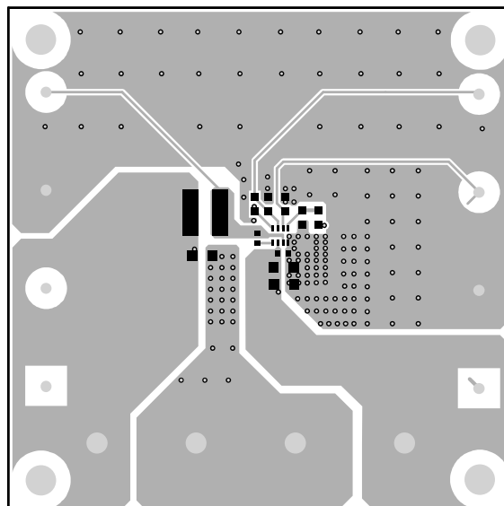
Figure 4: Top Layer
