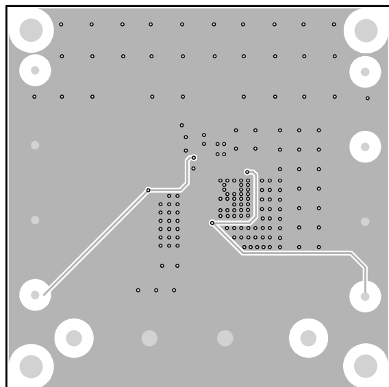
Figure 5: Bottom Layer
