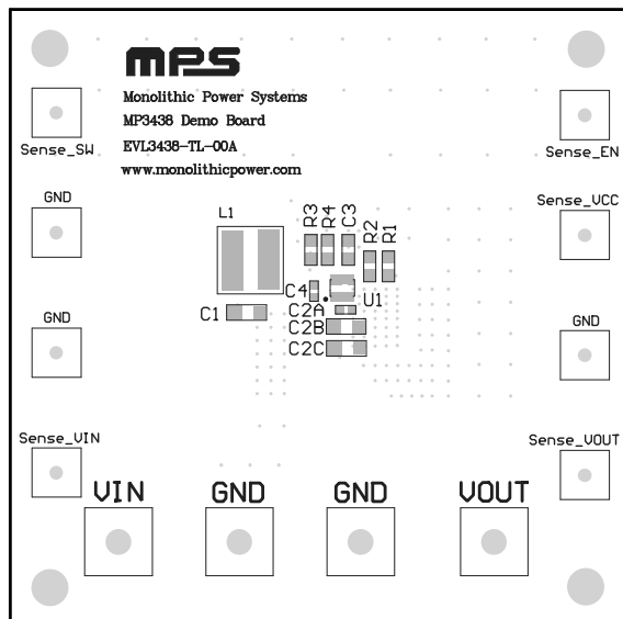
Figure 3: Top Silk
