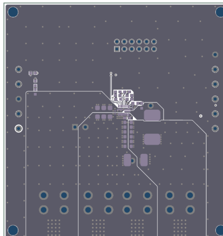
Figure 3: Top Layer
