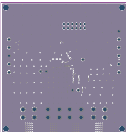
Figure 4: Mid-Layer 1
