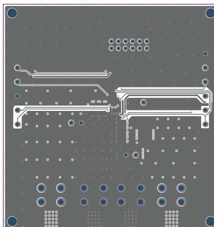
Figure 5: Mid-Layer 2
