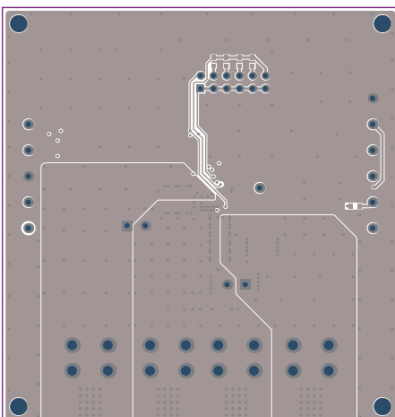
Figure 6: Bottom Layer
