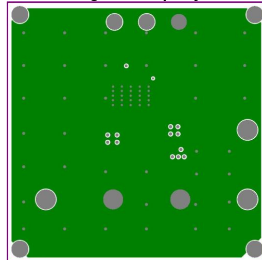
Figure 4: Inner1 Layer
