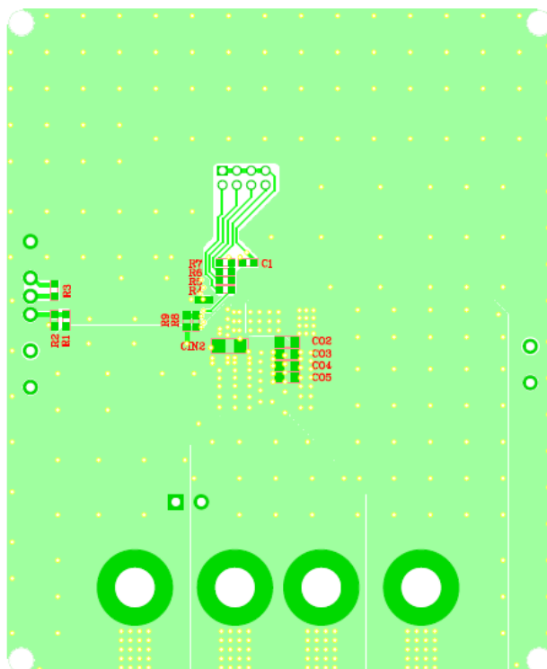
Figure 4: Bottom Layer
