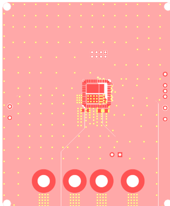
Figure 2: Top Layer
