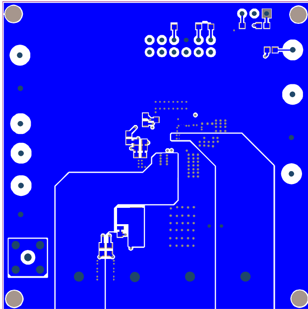
Figure 8: Bottom Layer
