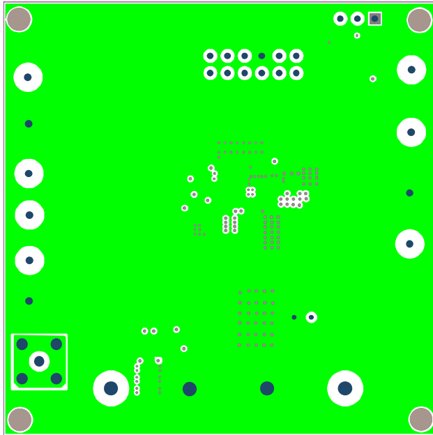
Figure 6: Mid-Layer 3
