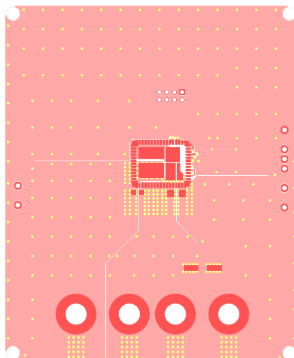
Figure 2: Top Layer
