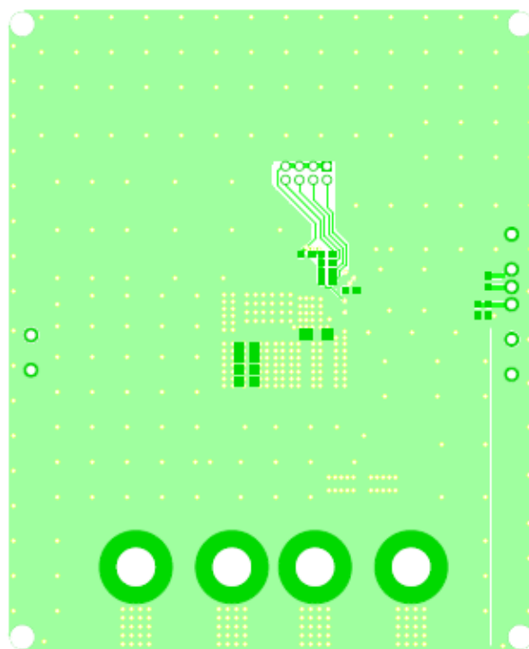
Figure 4: Bottom Layer
