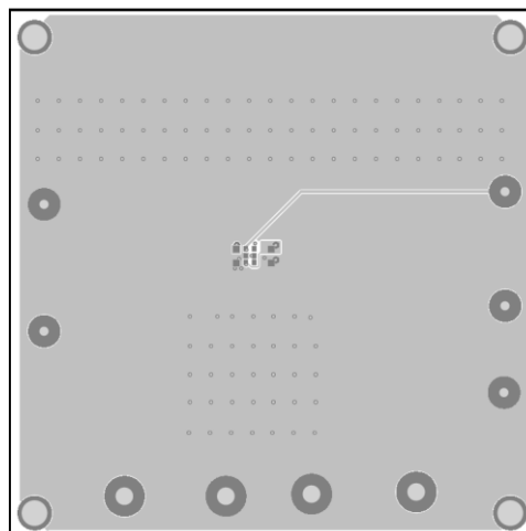
Figure 4: Bottom Layer
