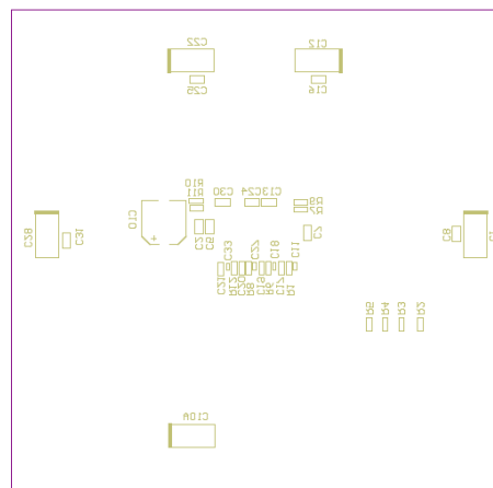
Figure 9: Bottom Silk
