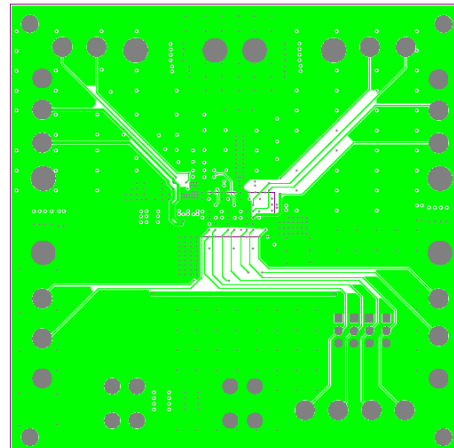
Figure 5: Mid-Layer 2
