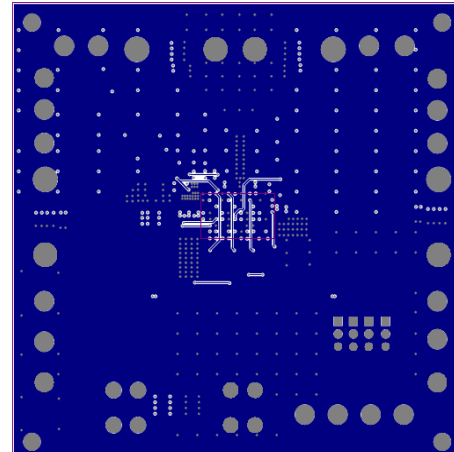
Figure 7: Mid-Layer 4
