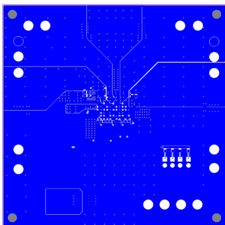
Figure 8: Bottom Layer
