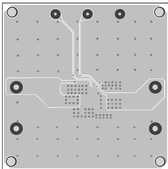
Figure 4: Mid-Layer 2
