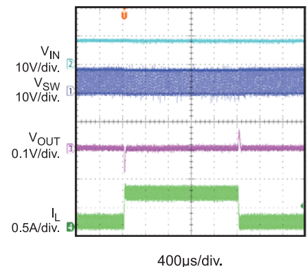
Load Transient
