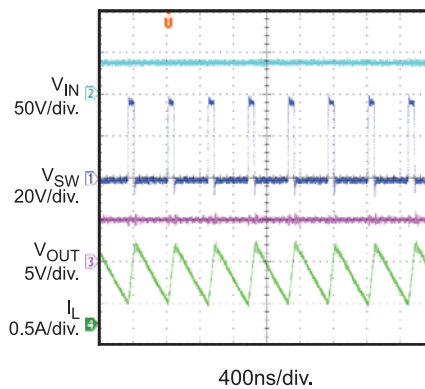
Steady State
