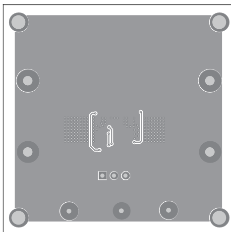
Figure 3: Bottom Layer
