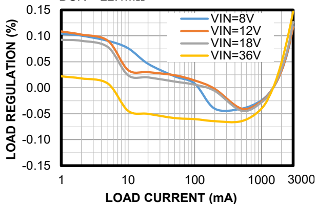
Load Regulation
