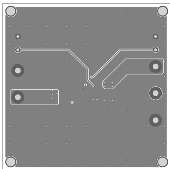
Figure 3: Inner2 Layer
