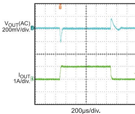
Load Transient Response I_{OUT} = 0A \text{ to } 1A, 1.6A/\mu s
