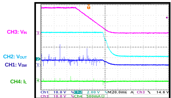
Shutdown through Input Voltage
