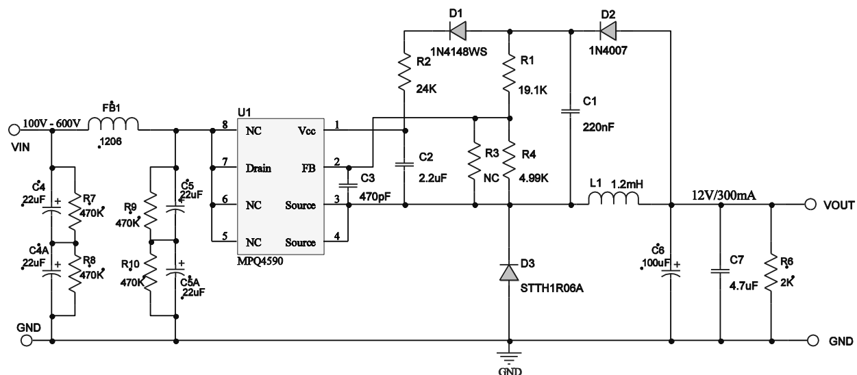
Figure 1—Schematic
