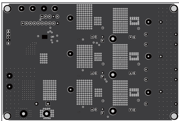
Figure 3: Inner1
