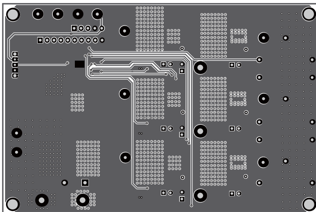
Figure 4: Inner2
