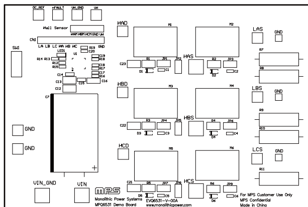
Figure 2: Top Silk
