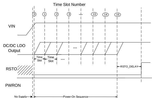
Figure 4: Power-On Sequence
