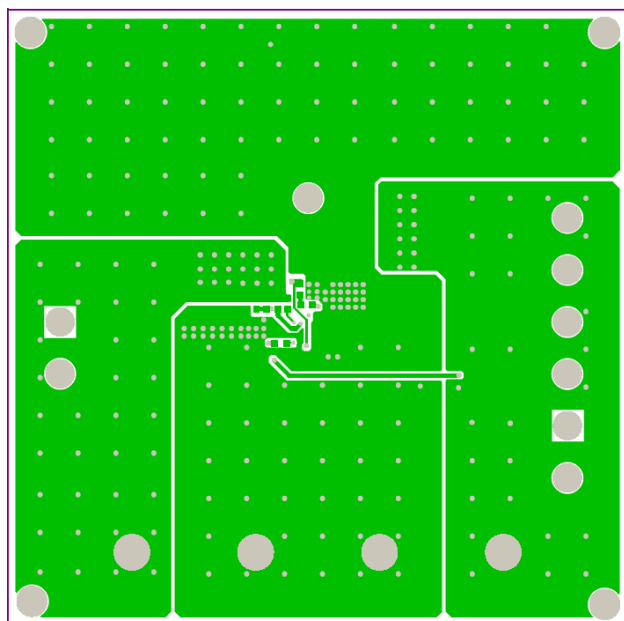
Figure 5: Bottom Layer
