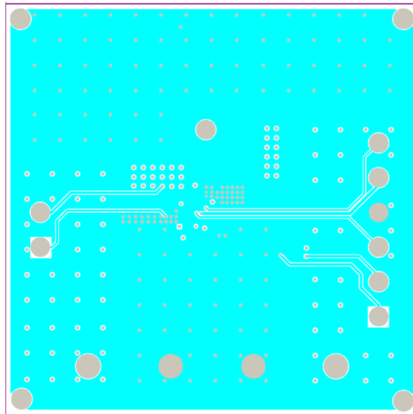
Figure 4: Inner Layer2
