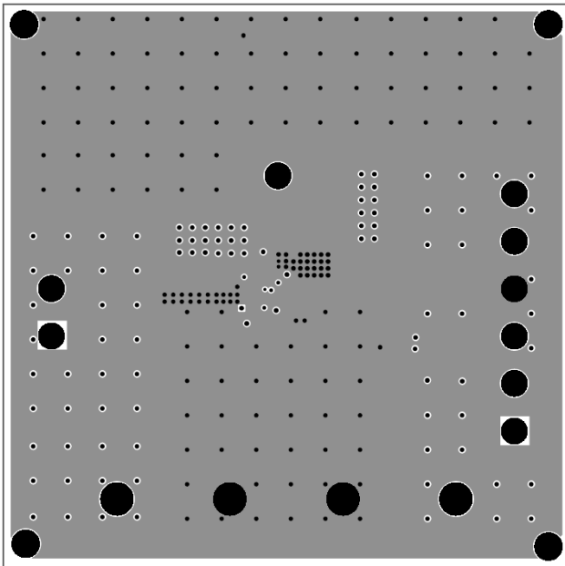
Figure 3: Inner Layer1
