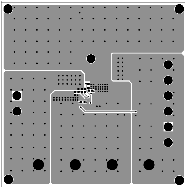
Figure 5: Bottom Layer
