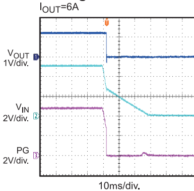
Power Good Through Shutdown I_{OUT} = 6A
