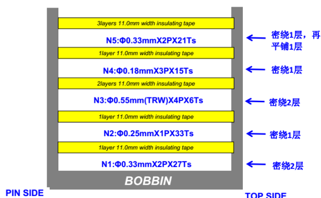
Figure 6: Winding Diagram
