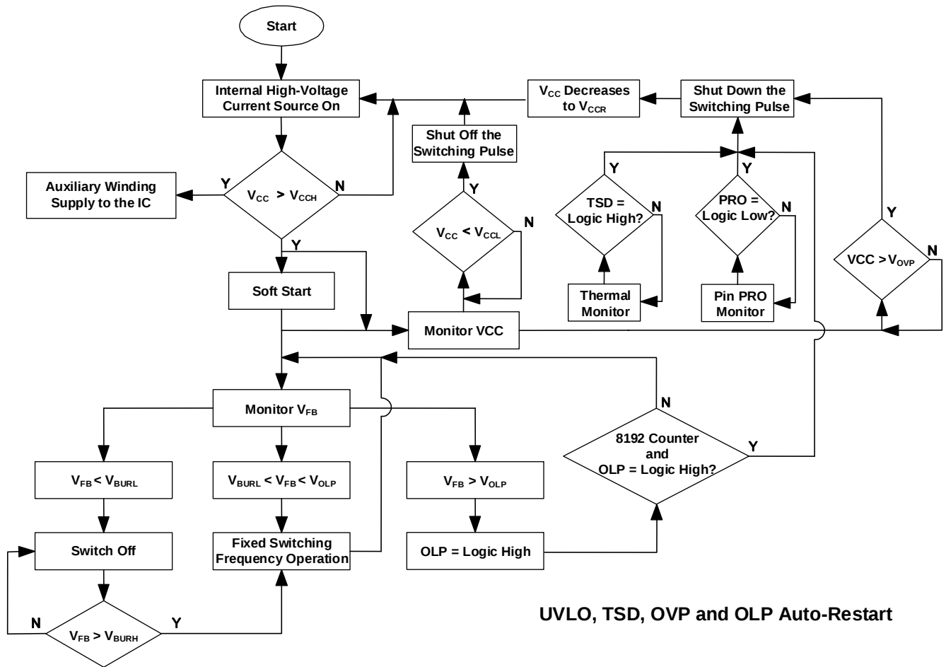
Figure 13: Control Flowchart
