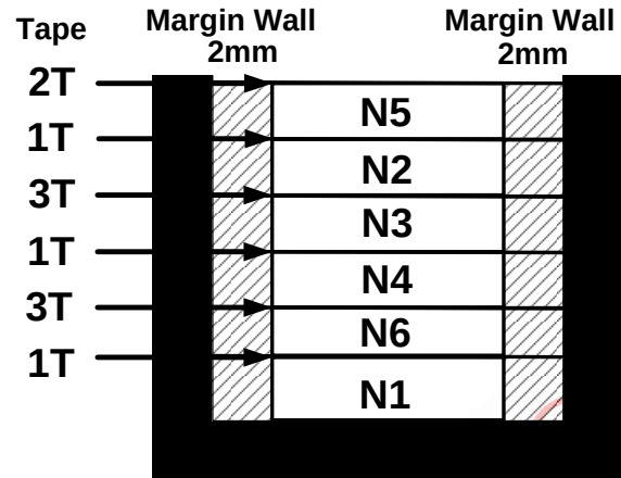
Bobbin
