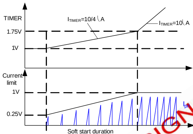
Figure 6: Soft-Start
