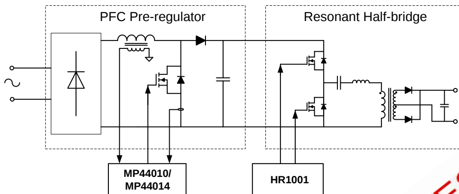
Figure 24: Application Circuit
