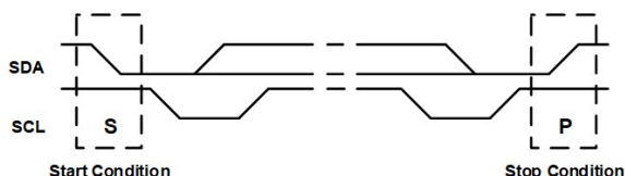
Figure 5: Start and Stop Conditions
