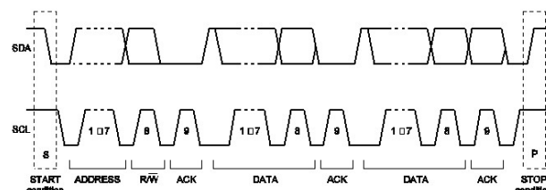
Figure 7: A Complete Data Transfer
