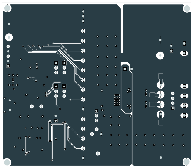
Figure 9: Bottom Layer
