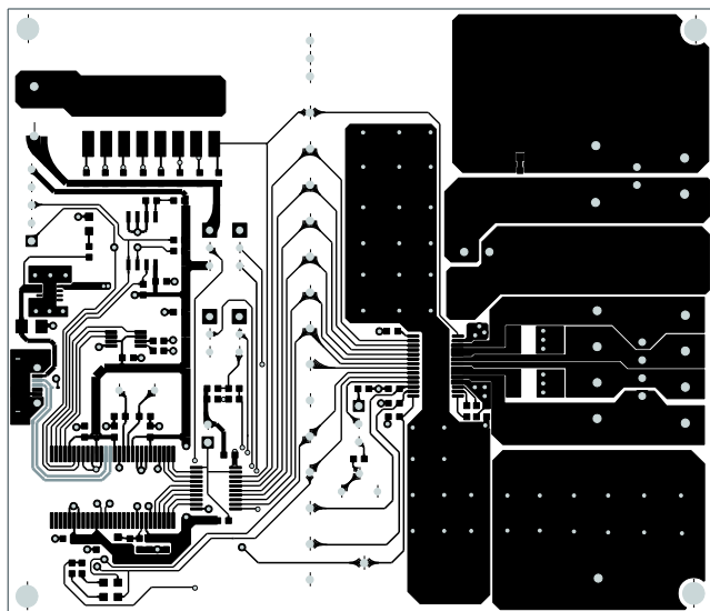
Figure 8: Top Layer
