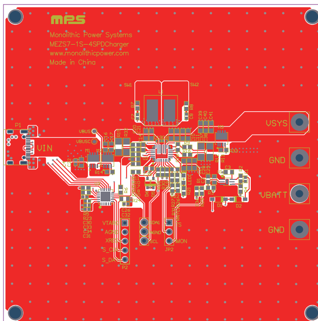
Figure 4: Top Layer
