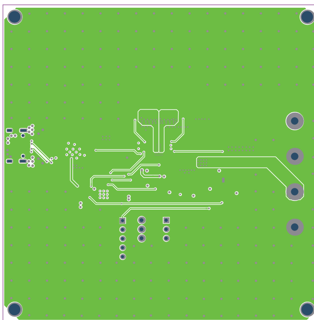
Figure 6: Mid-Layer 2
