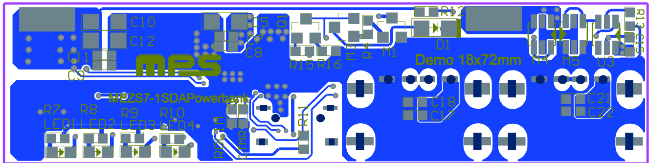
Figure 6: Bottom Layer
